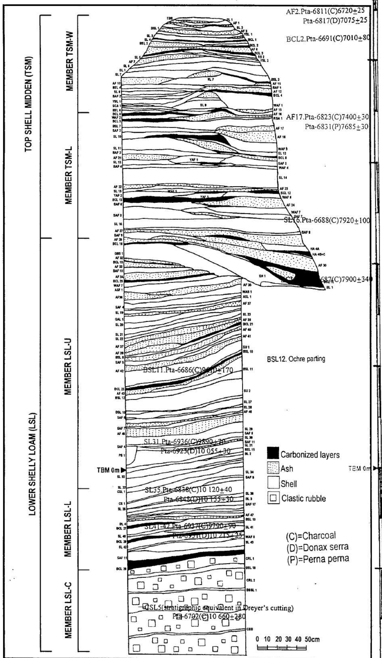
Figure 9: Stratigraphy of the Apex section
