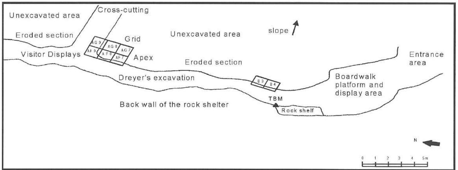
Figure 2: Plan of Matjes River rock shelter (after Döckel 1998)
